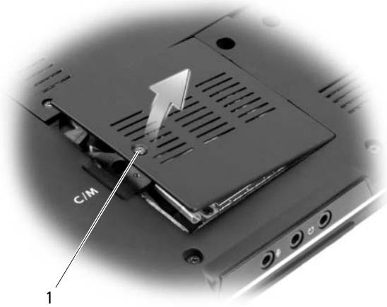
1 captive screw
